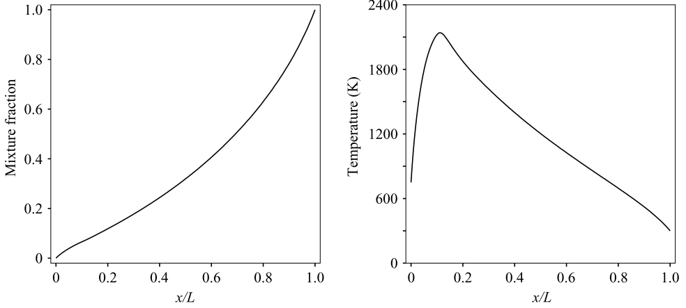
FIGURE 1. Mixture fraction and temperature from a steady-flamelet solution in physical space. Methane–air combustion at the conditions of the experiment in §5 (750 K air, 300 K fuel, 3.8 atm). L = 0.2 cm.
