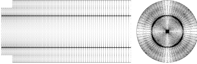
FIGURE 5. Schematic of the grid used for the simulations. Only half of the points in the axial and radial directions are shown for clarity.
